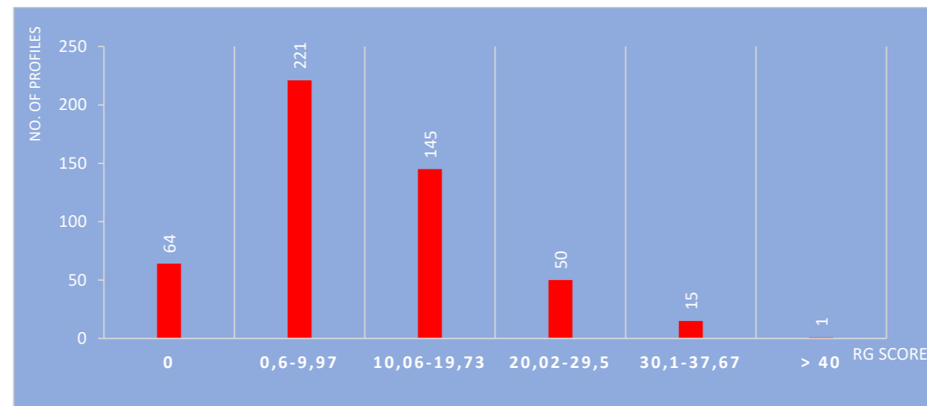
Fig. 1. RG Score distribution related to academic staff
