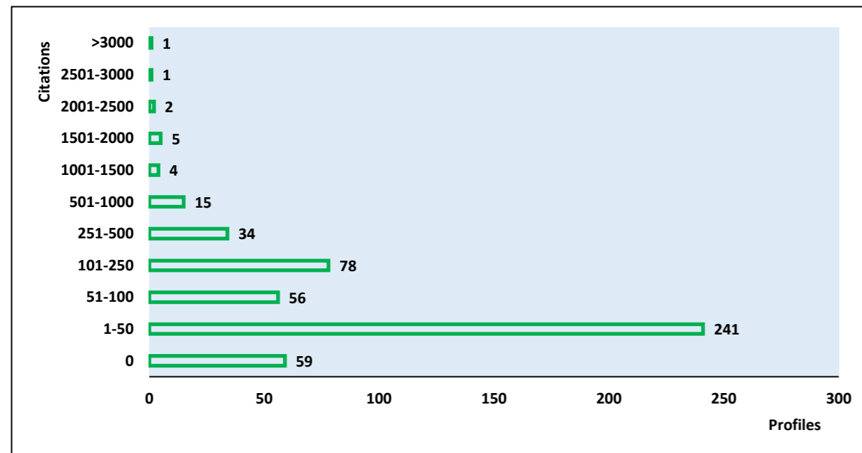
Fig. 2 Academic staff distribution, by citations
