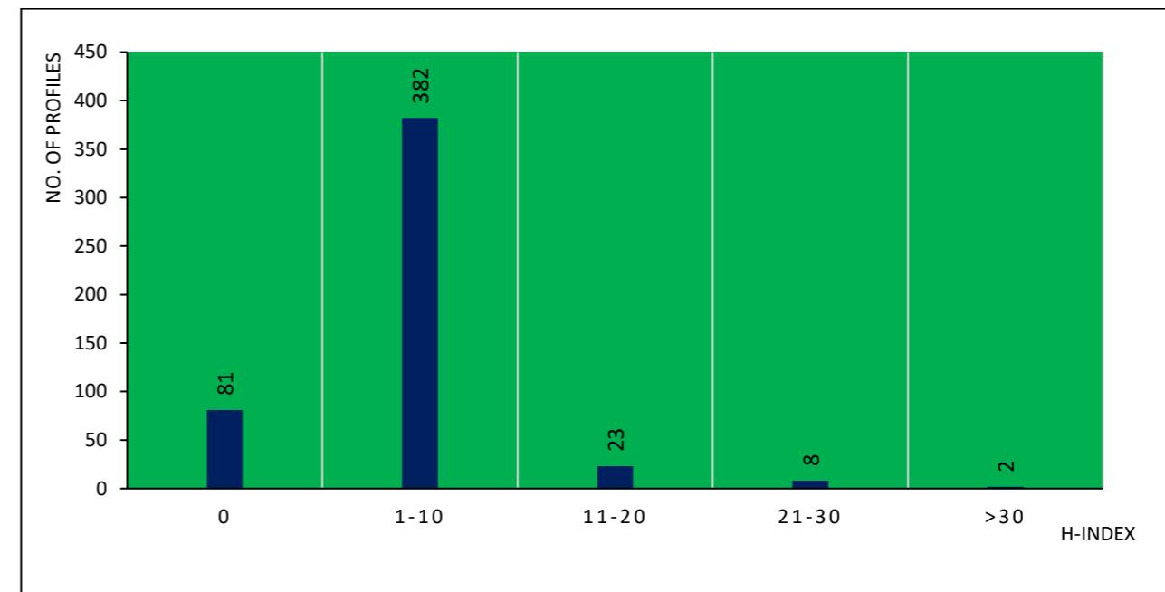
Fig. 3 Academic staff distribution, by H-index
